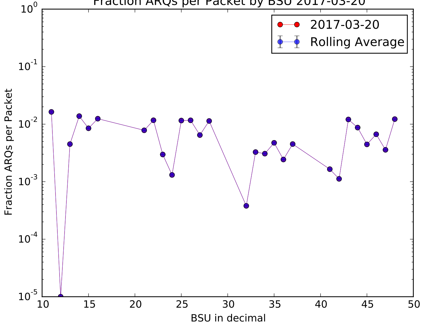
Fraction ARQs per Packet by BSU 2017-03-20
