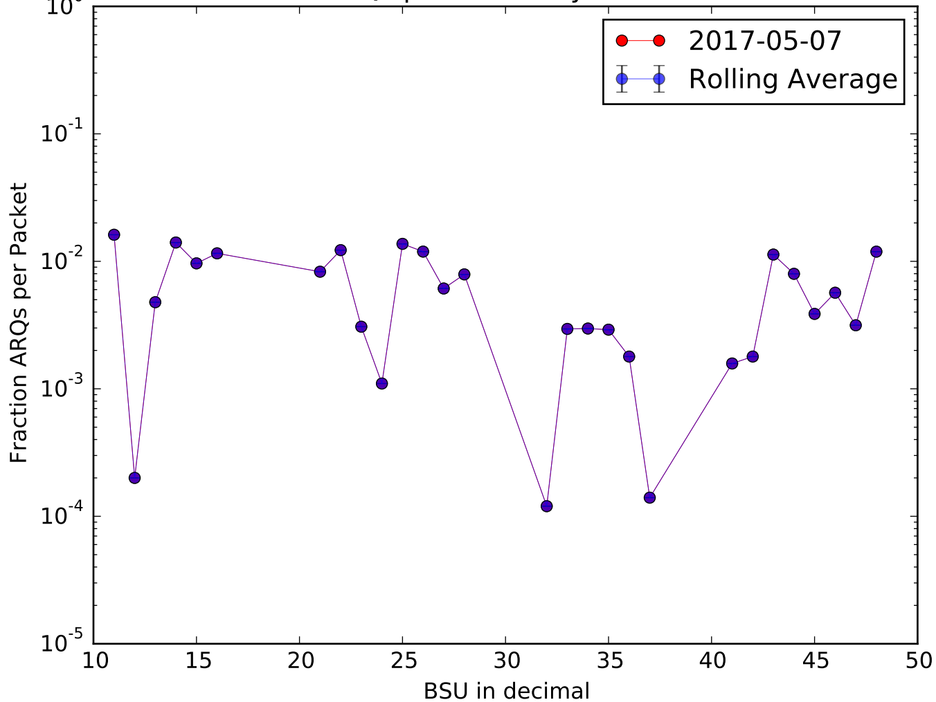
Fraction ARQs per Packet by BSU 2017-05-07
