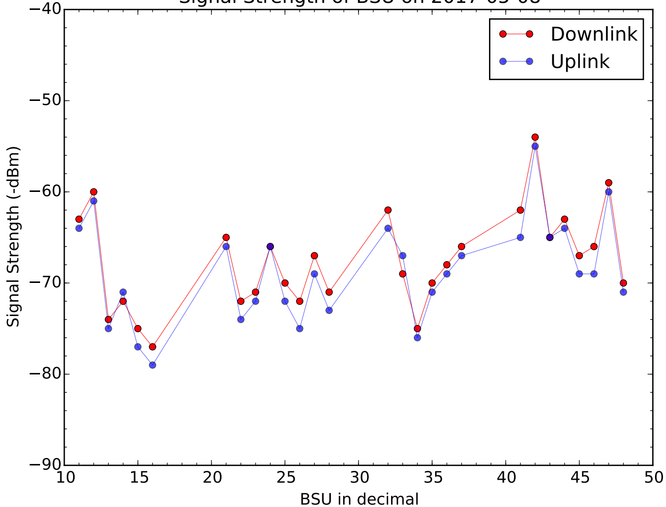
Signal Strength of BSU on 2017-05-08
