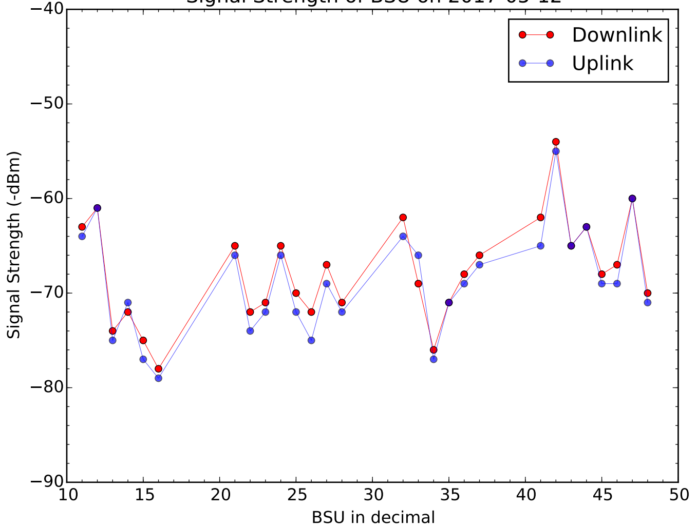
Signal Strength of BSU on 2017-05-12
