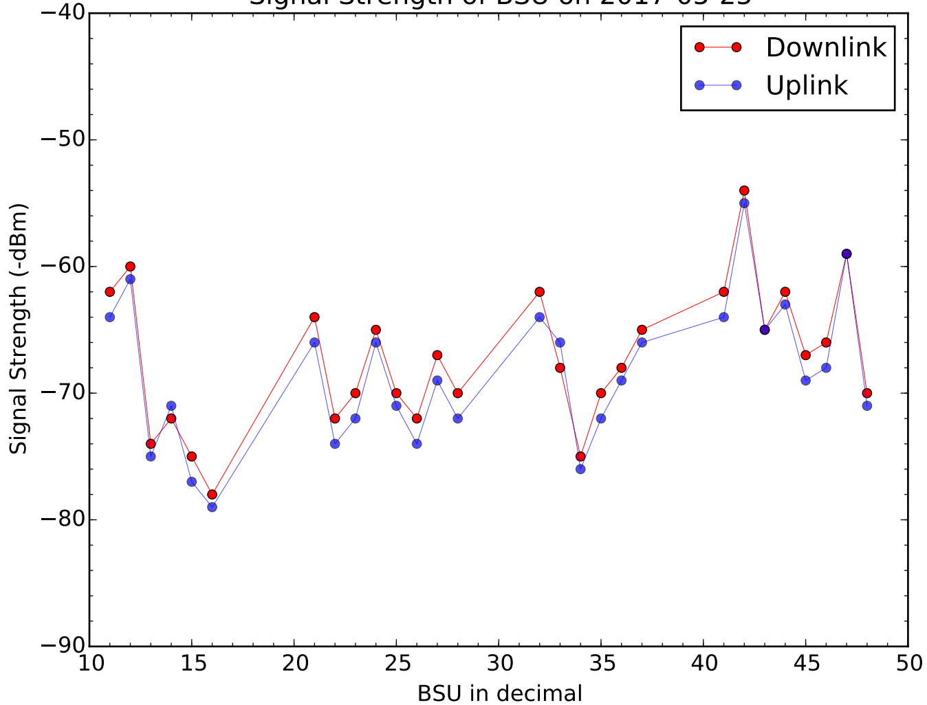
Signal Strength of BSU on 2017-05-25
