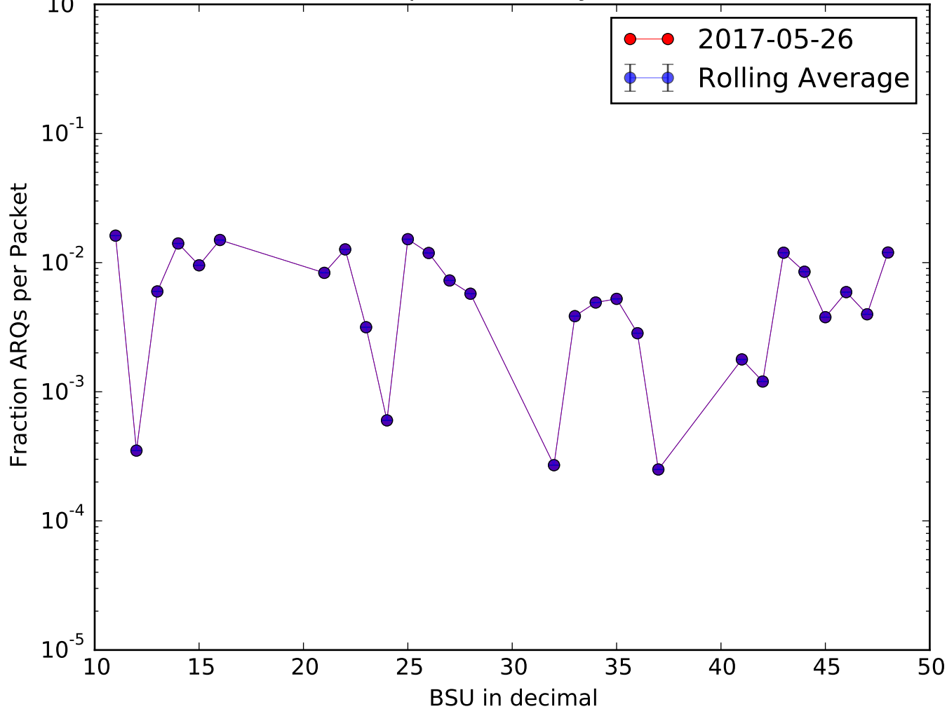
Fraction ARQs per Packet by BSU 2017-05-26
