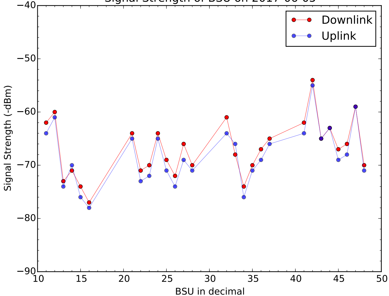
Signal Strength of BSU on 2017-06-05
