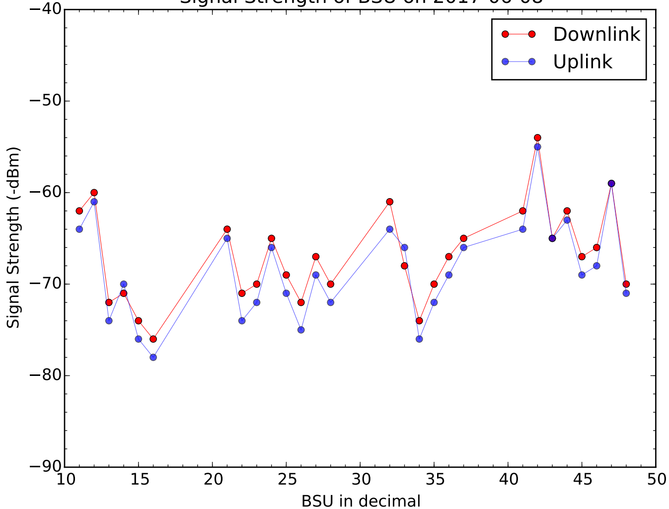
Signal Strength of BSU on 2017-06-08
