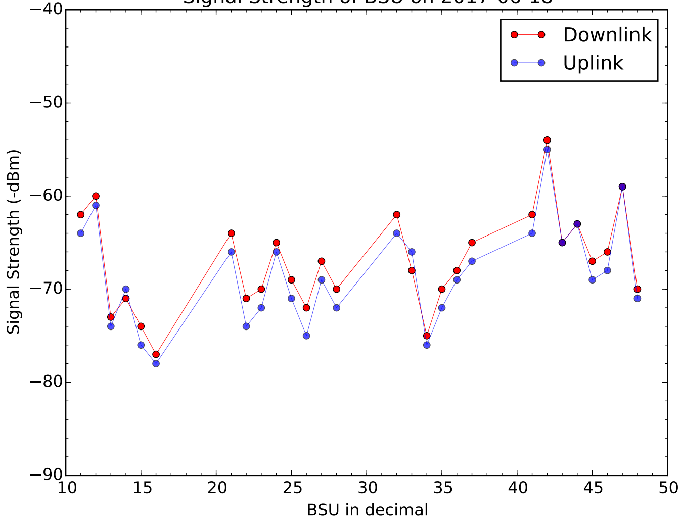
Signal Strength of BSU on 2017-06-18
