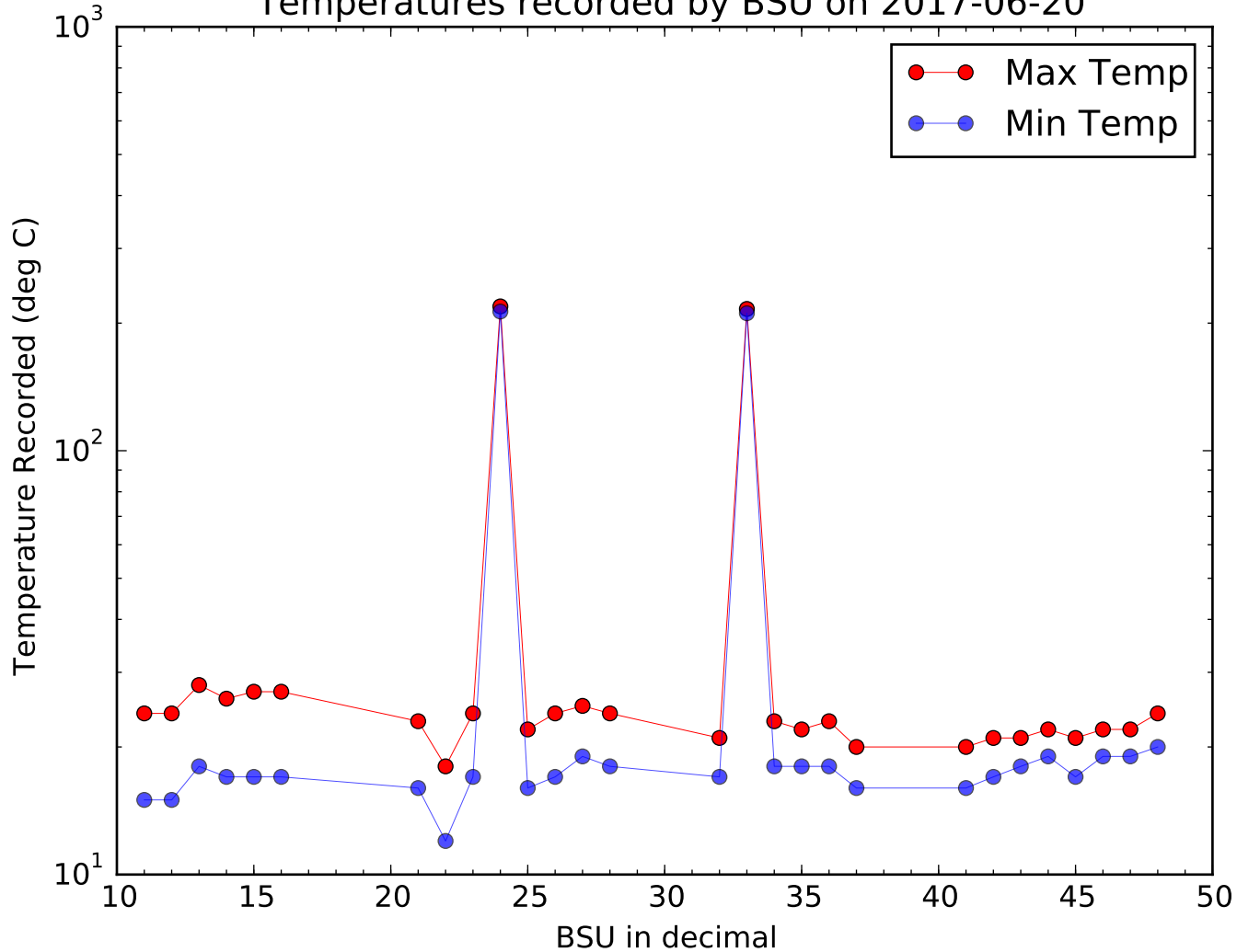
Temperatures recorded by BSU on 2017-06-20
