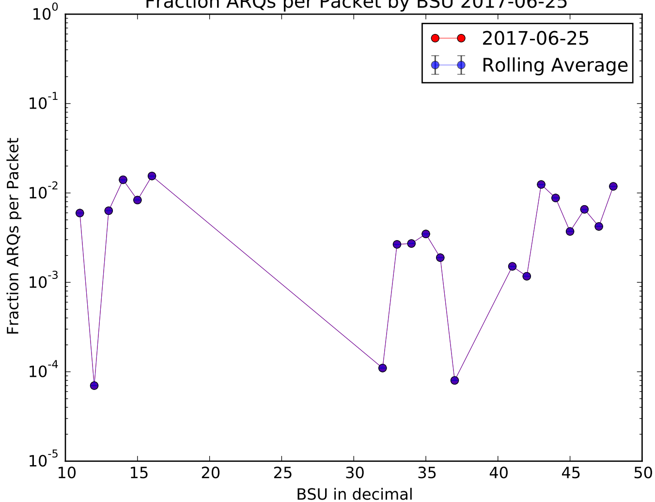
Fraction ARQs per Packet by BSU 2017-06-25
