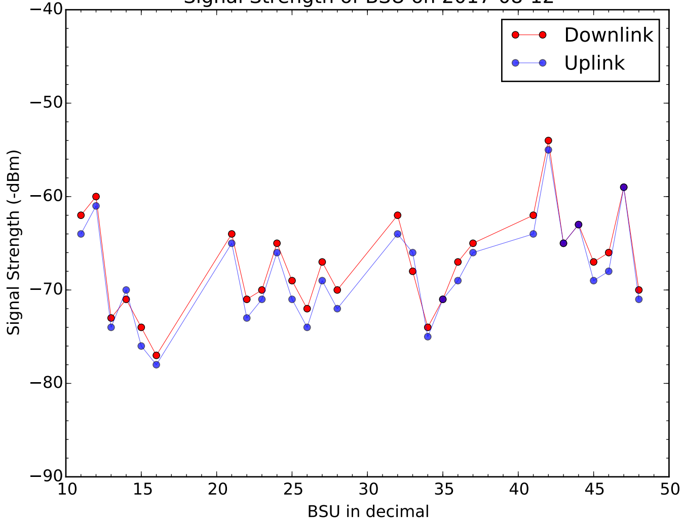
Signal Strength of BSU on 2017-08-12
