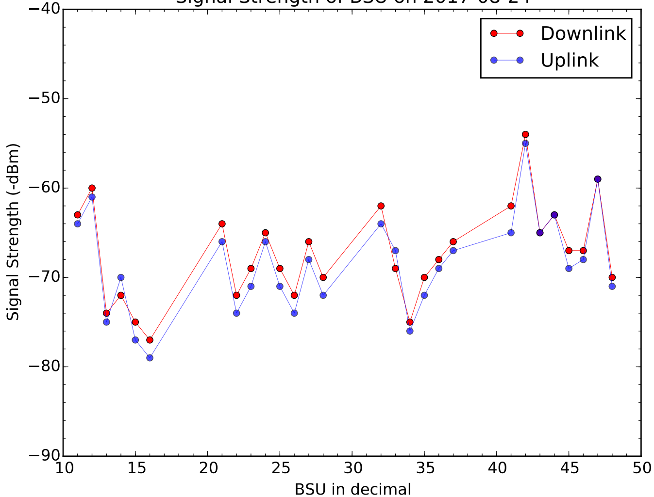
Signal Strength of BSU on 2017-08-24
