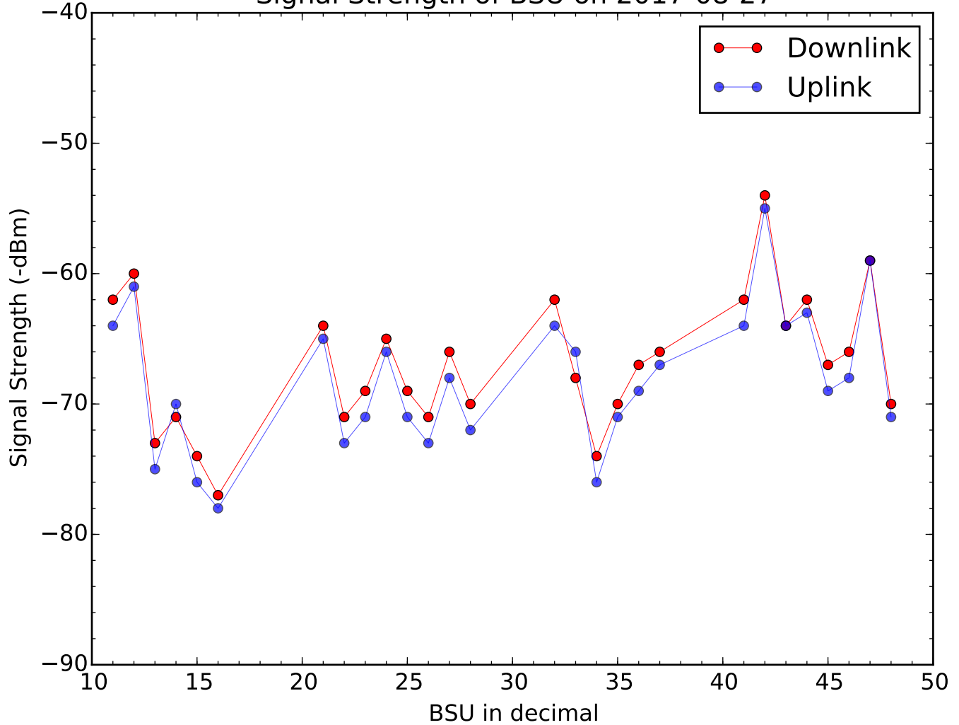
Signal Strength of BSU on 2017-08-27
