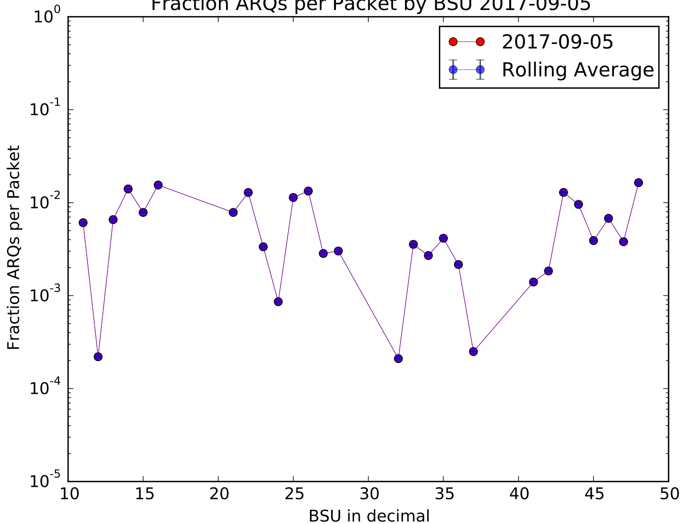
Fraction ARQs per Packet by BSU 2017-09-05
