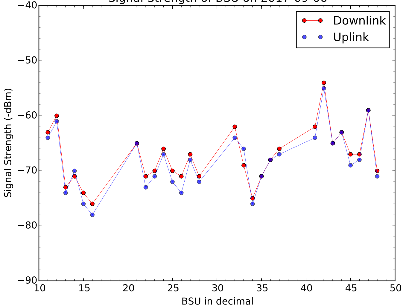
Signal Strength of BSU on 2017-09-06
