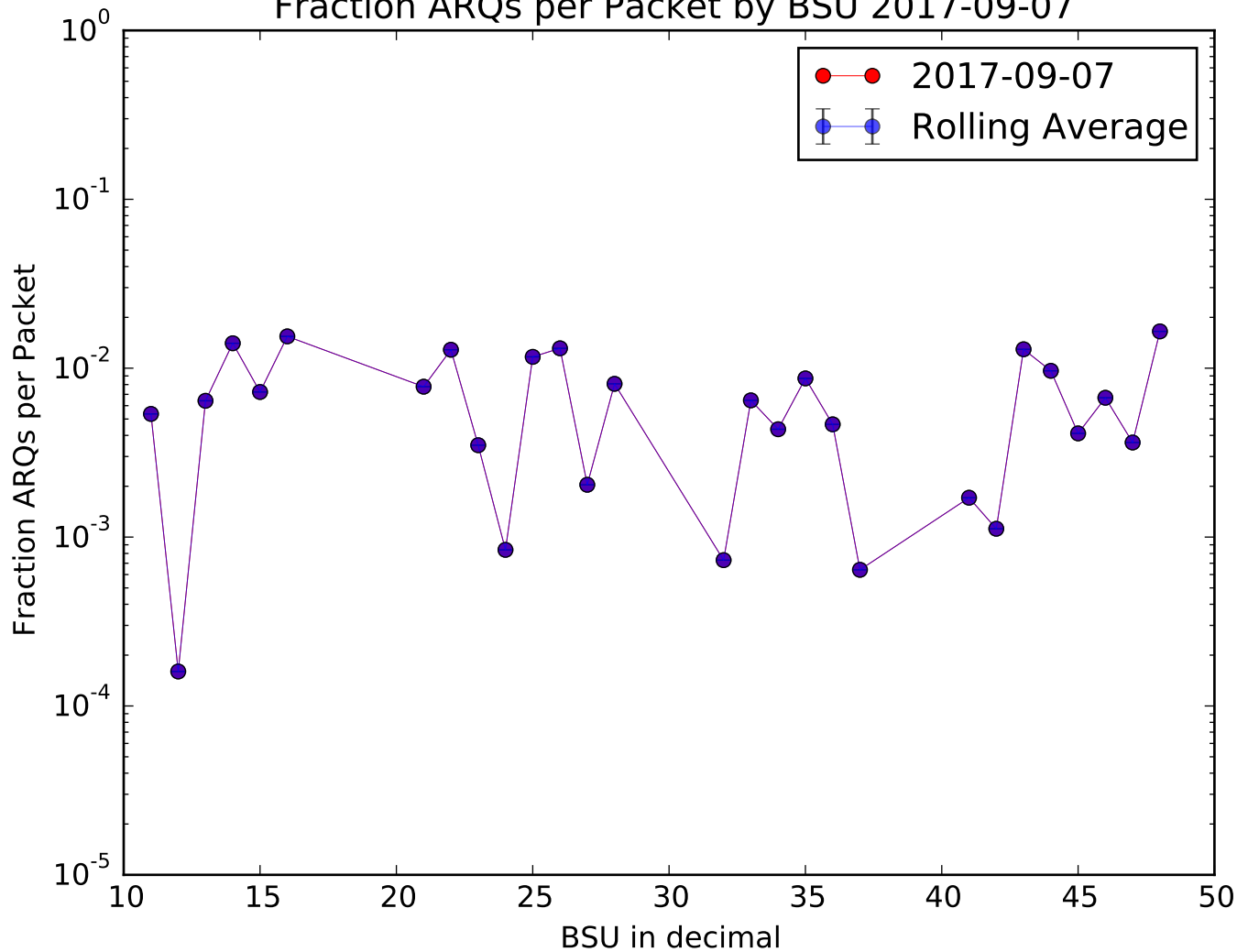
Fraction ARQs per Packet by BSU 2017-09-07
