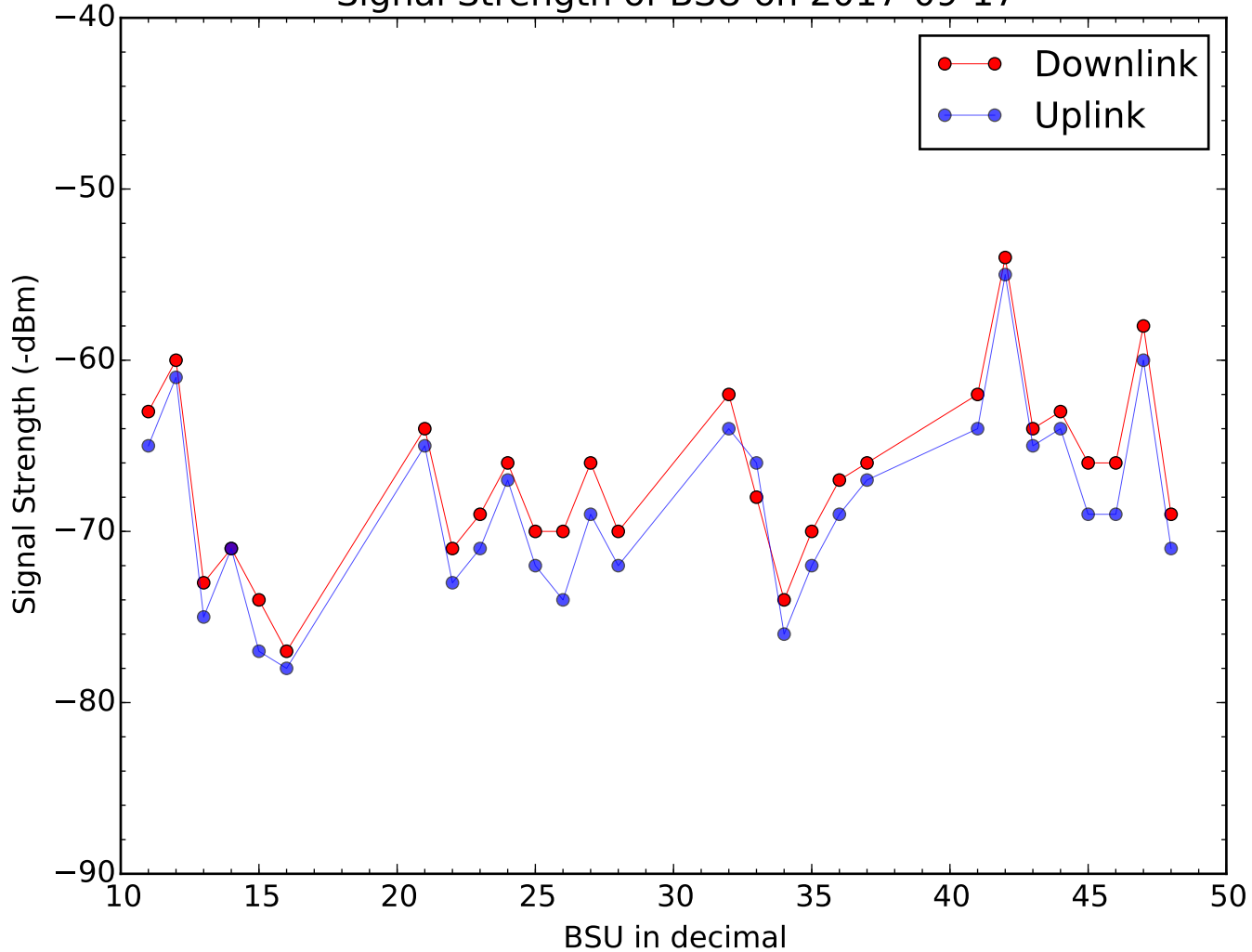
Signal Strength of BSU on 2017-09-17
