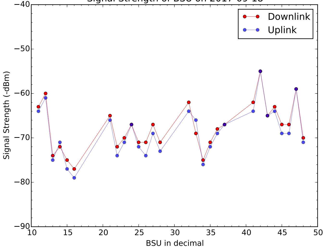
Signal Strength of BSU on 2017-09-18
