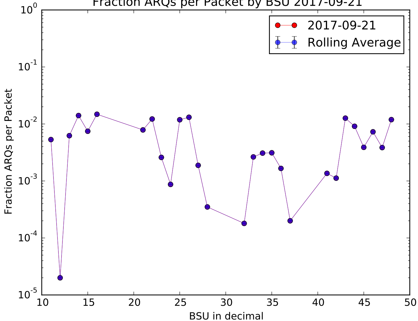
Fraction ARQs per Packet by BSU 2017-09-21
