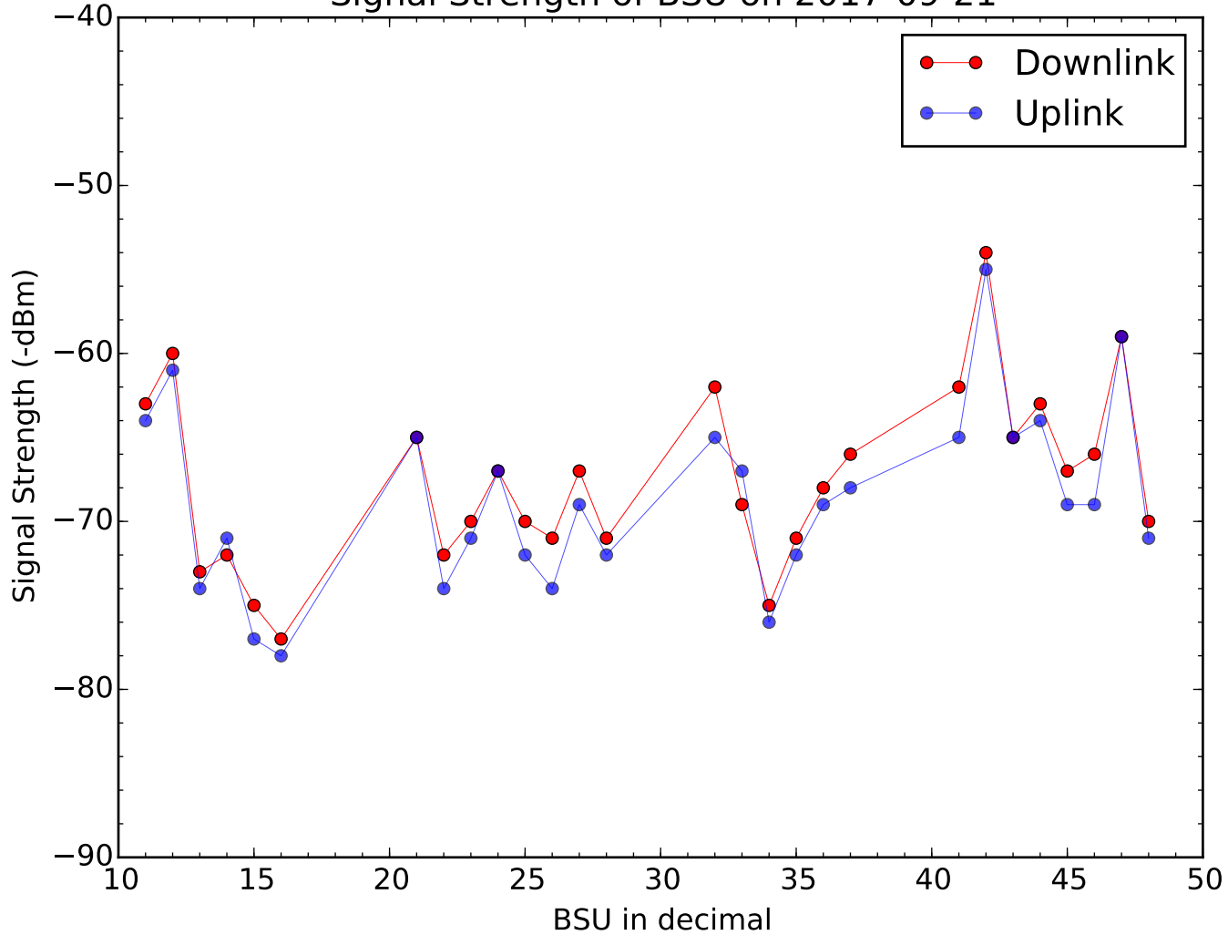
Signal Strength of BSU on 2017-09-21
