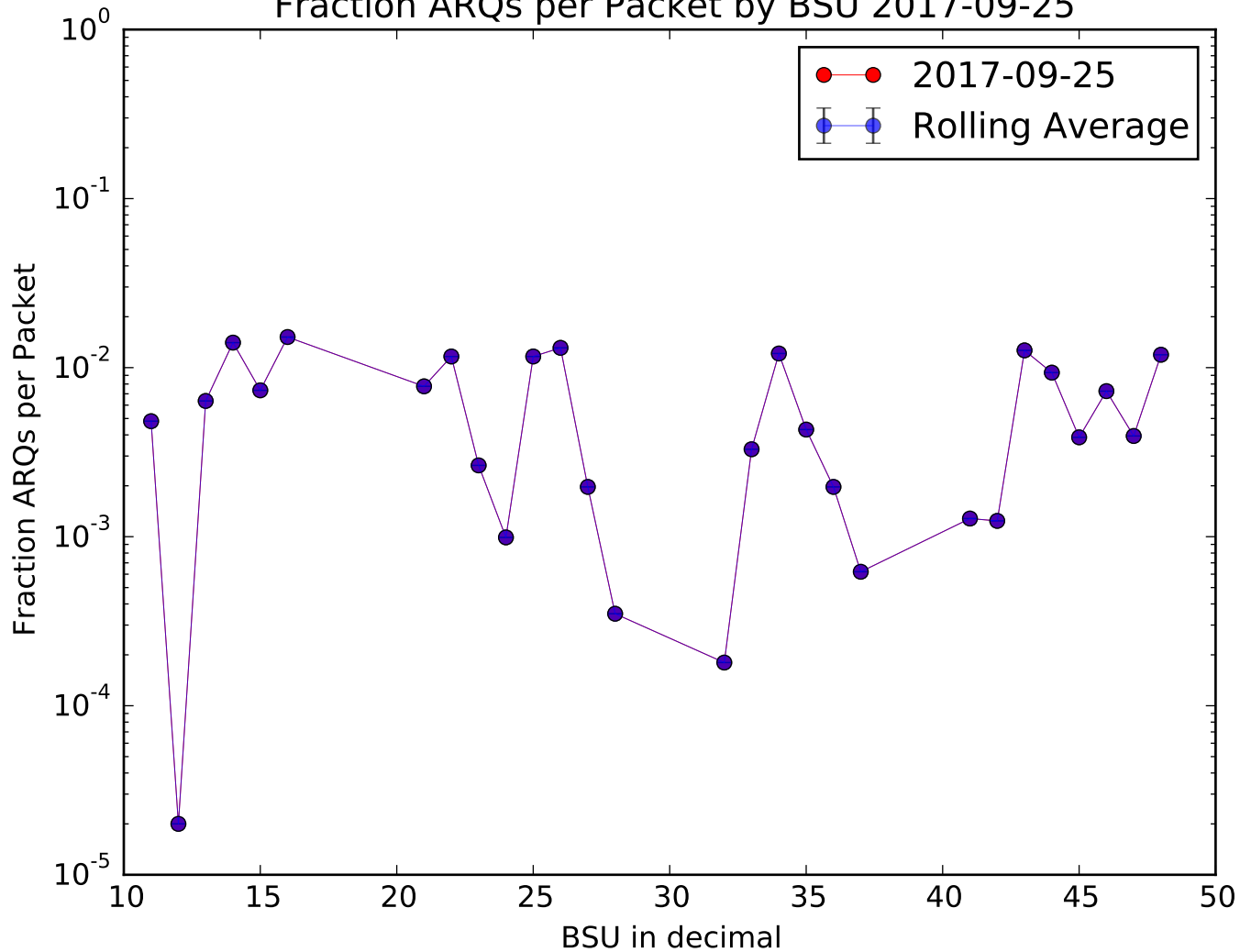
Fraction ARQs per Packet by BSU 2017-09-25
