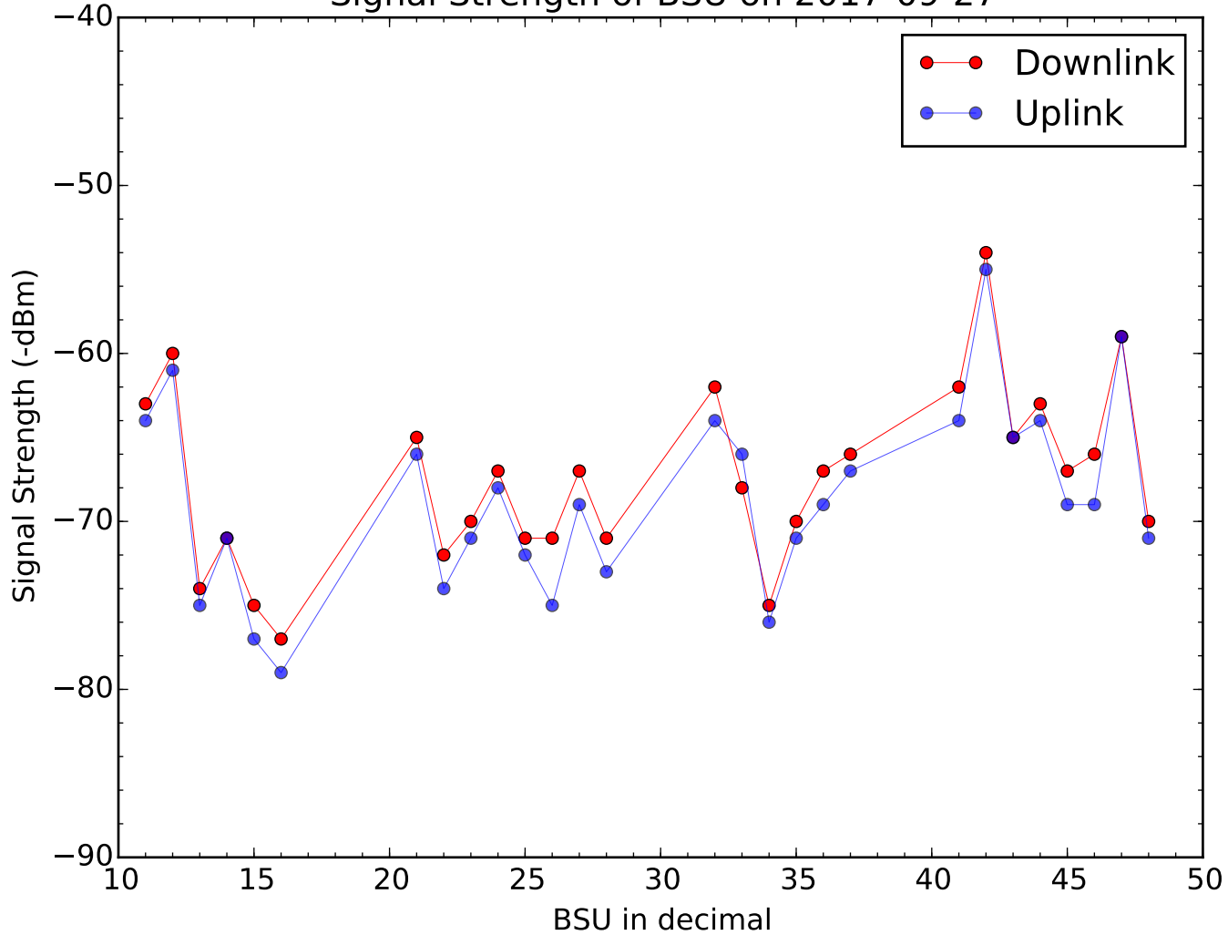
Signal Strength of BSU on 2017-09-27
