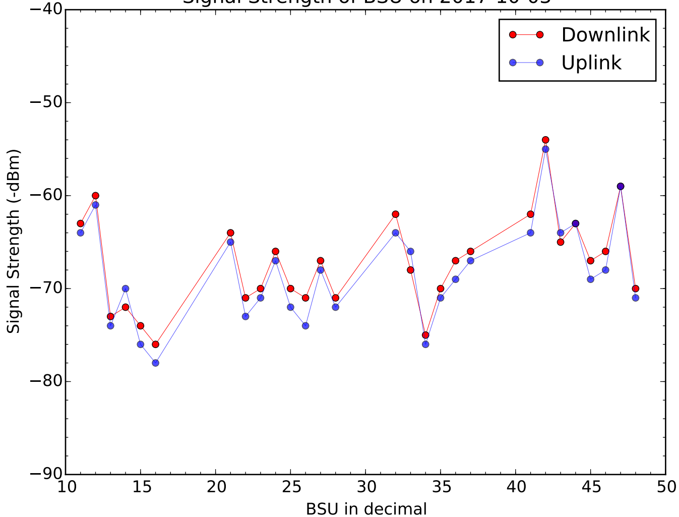
Signal Strength of BSU on 2017-10-03
