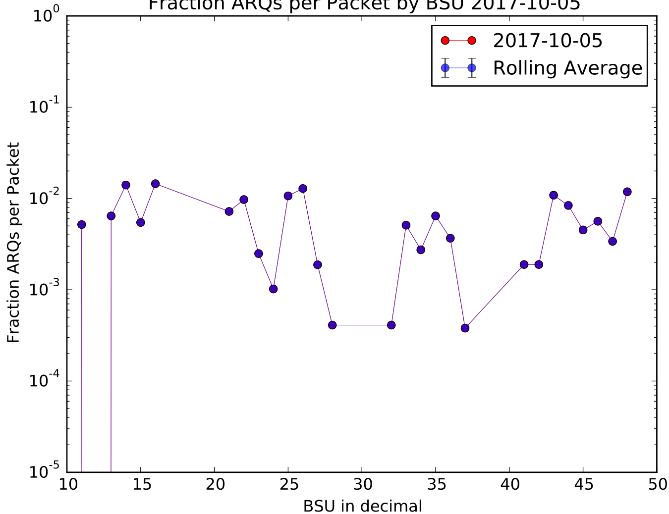
Fraction ARQs per Packet by BSU 2017-10-05
