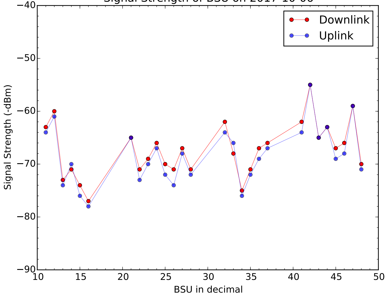
Signal Strength of BSU on 2017-10-06
