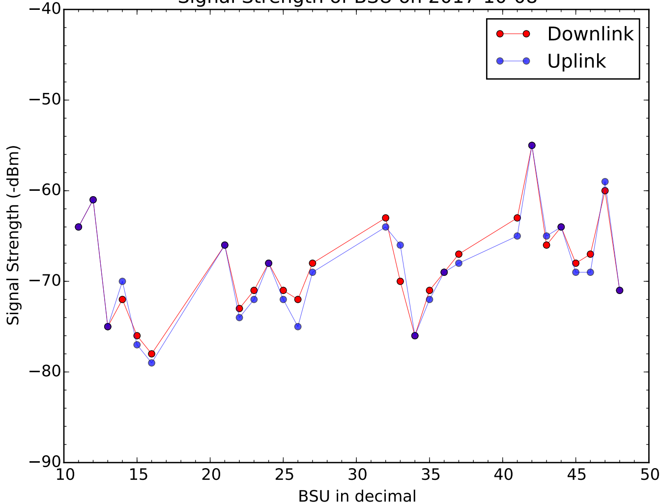
Signal Strength of BSU on 2017-10-08
