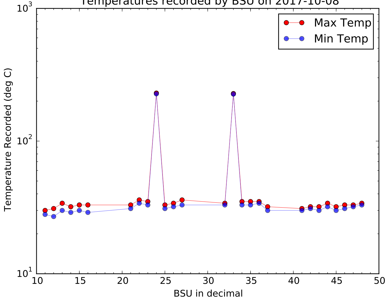
Temperatures recorded by BSU on 2017-10-08
