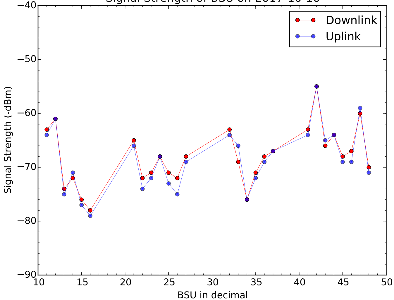
Signal Strength of BSU on 2017-10-10
