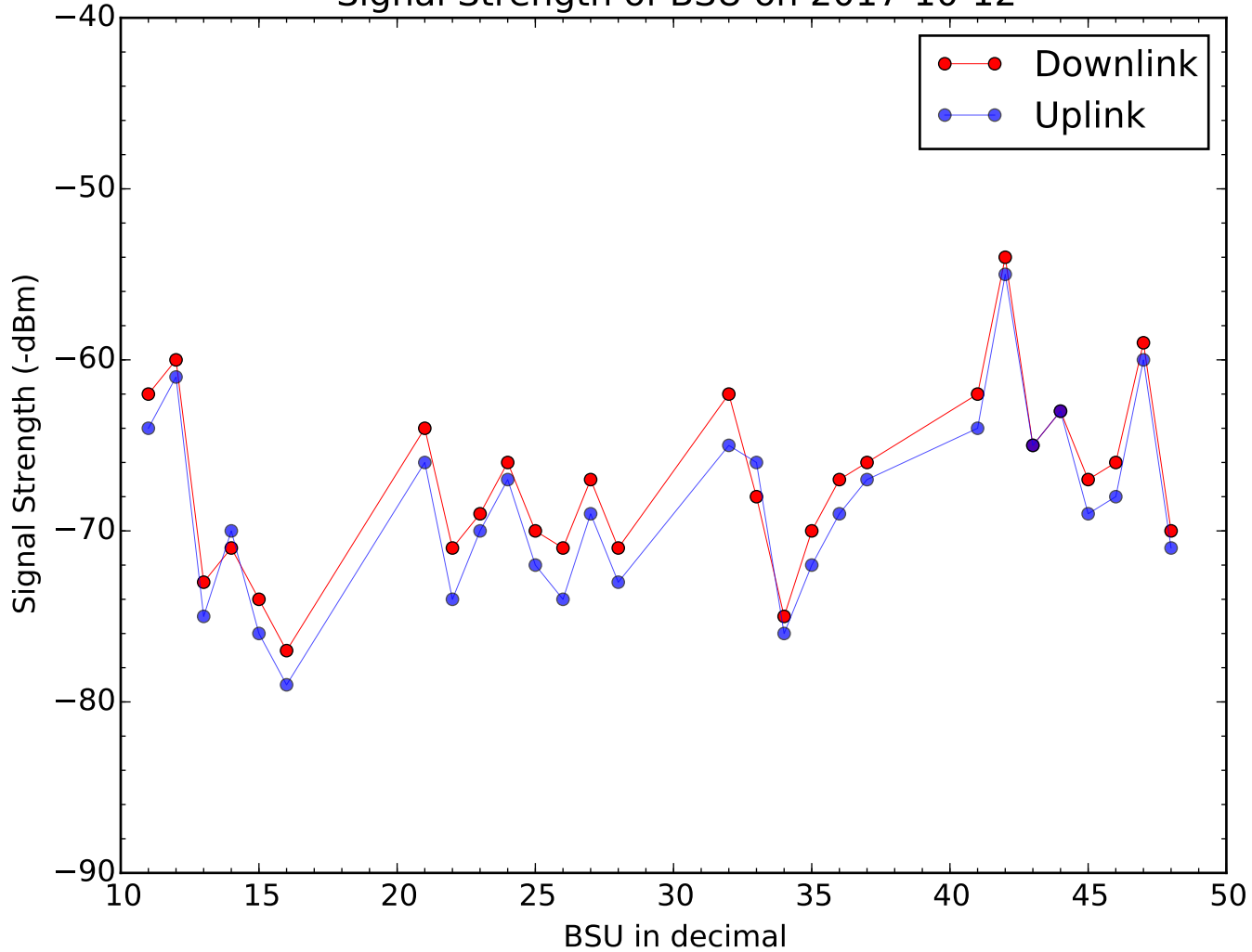
Signal Strength of BSU on 2017-10-12
