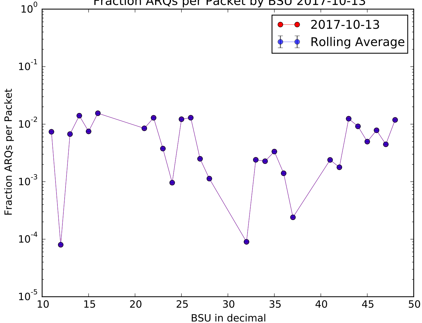
Fraction ARQs per Packet by BSU 2017-10-13
