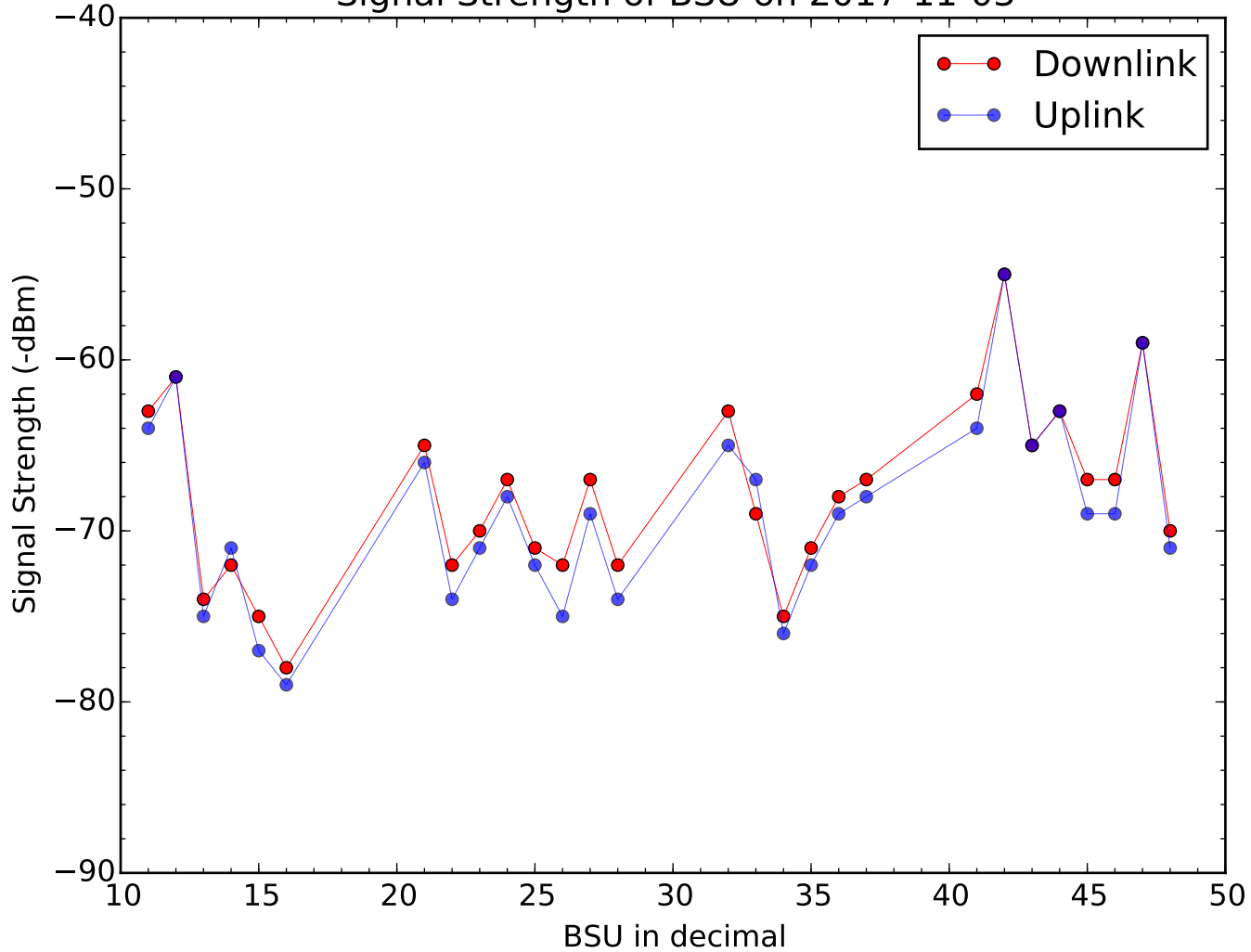
Signal Strength of BSU on 2017-11-03
