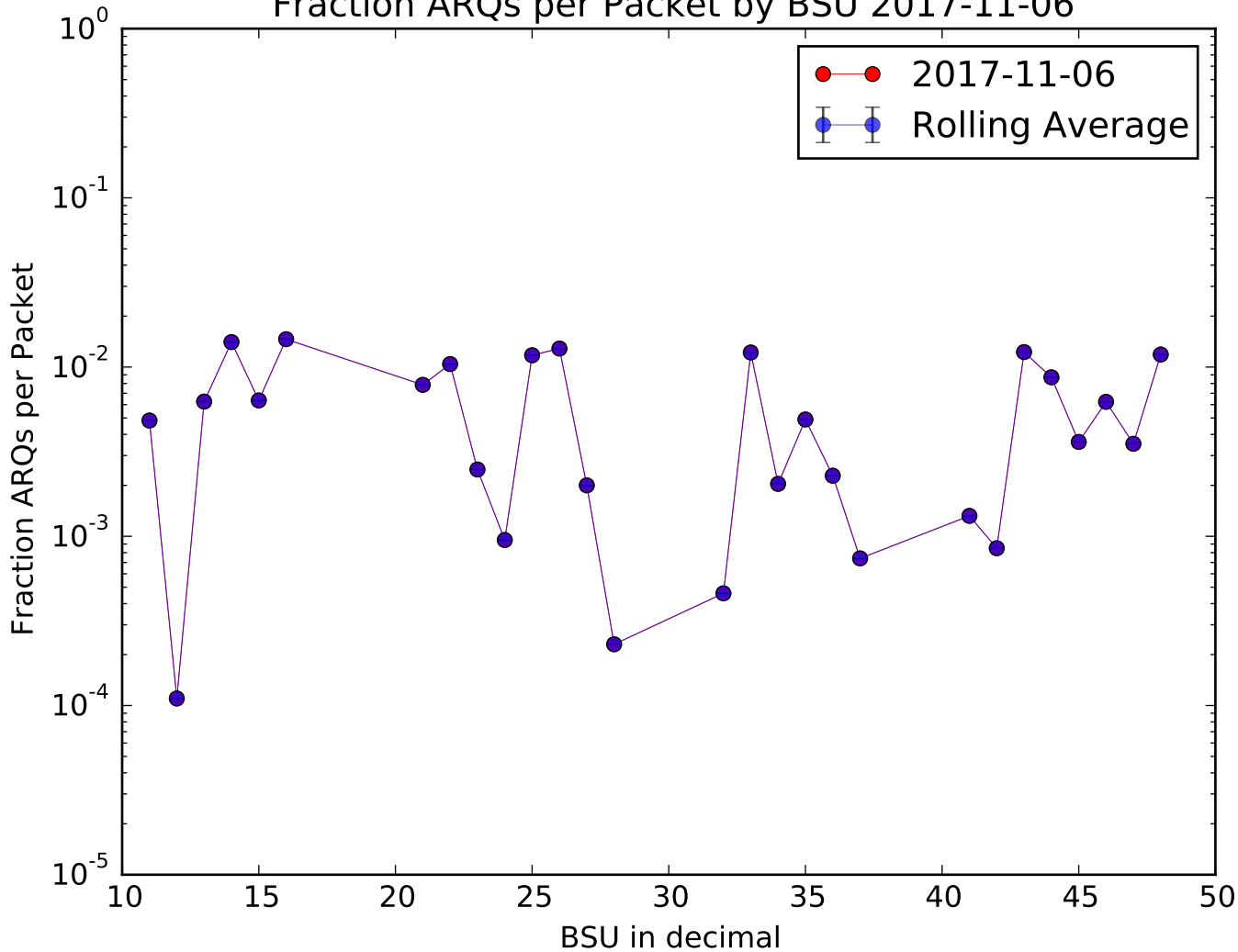
Fraction ARQs per Packet by BSU 2017-11-06
