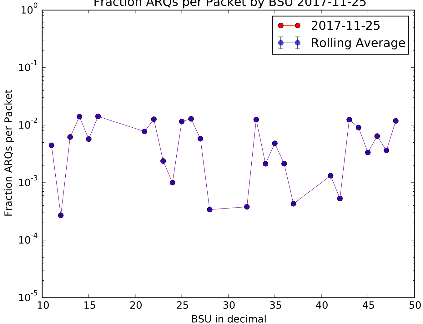
Fraction ARQs per Packet by BSU 2017-11-25
