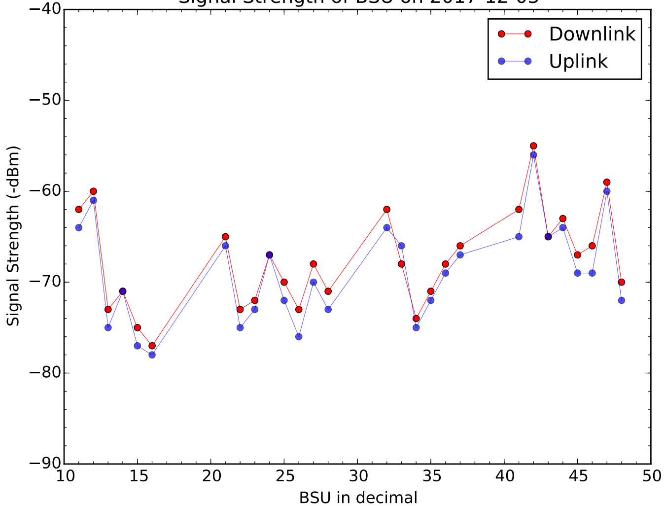
Signal Strength of BSU on 2017-12-03
