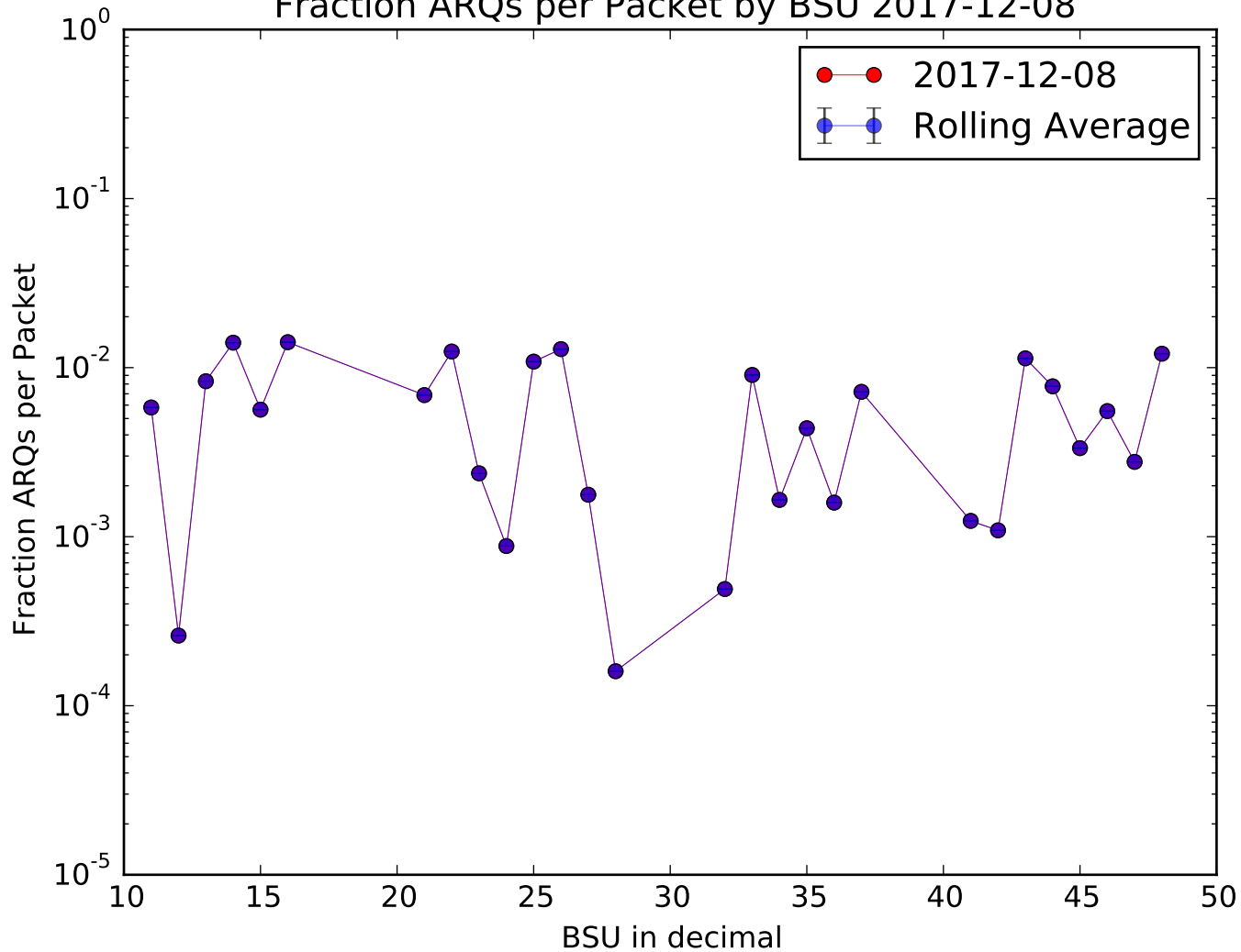
Fraction ARQs per Packet by BSU 2017-12-08
