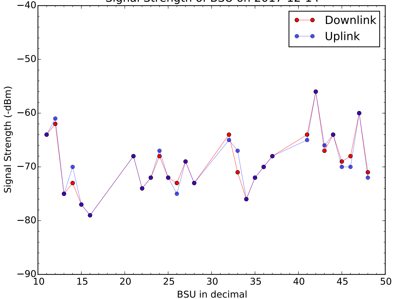
Signal Strength of BSU on 2017-12-14
