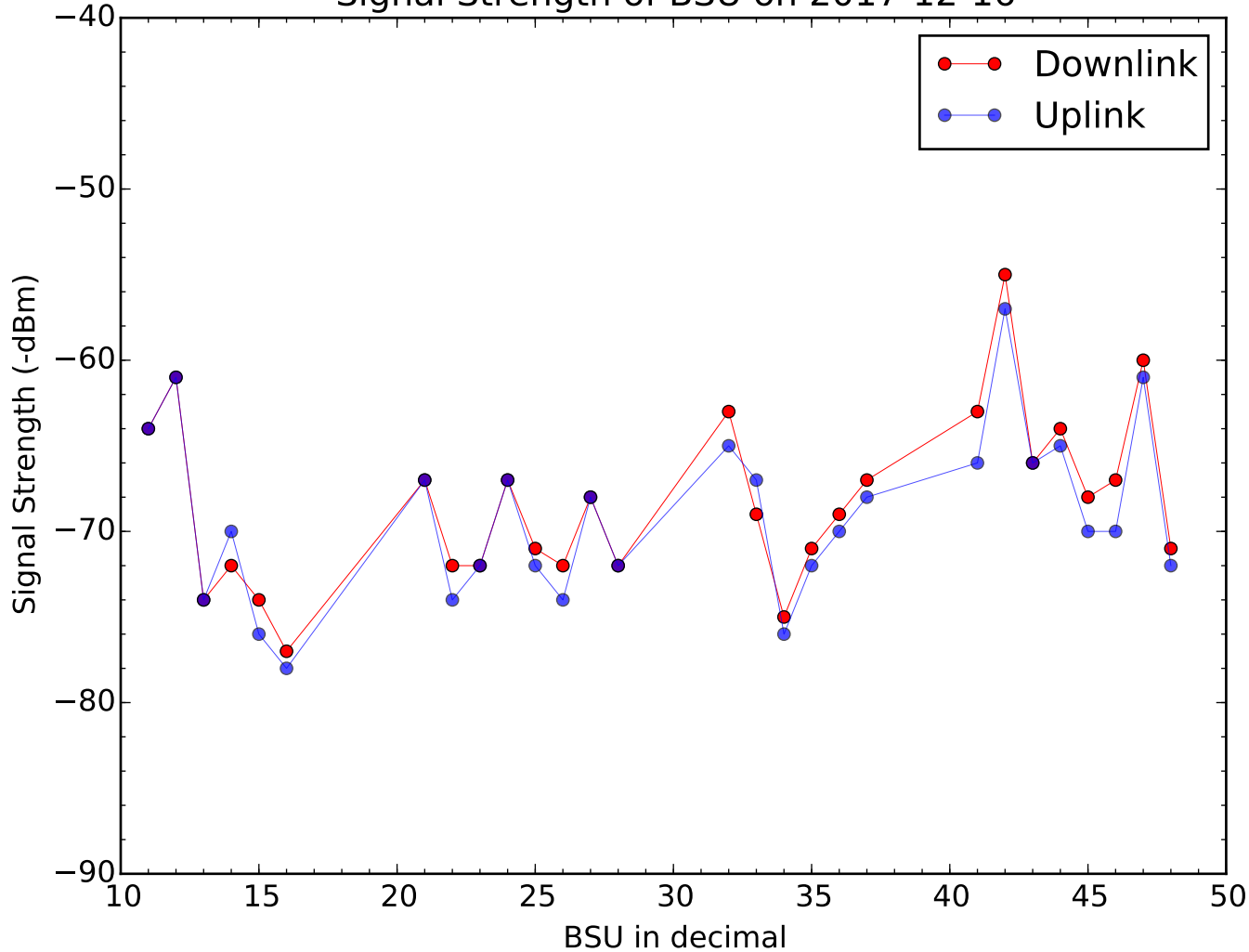
Signal Strength of BSU on 2017-12-16
