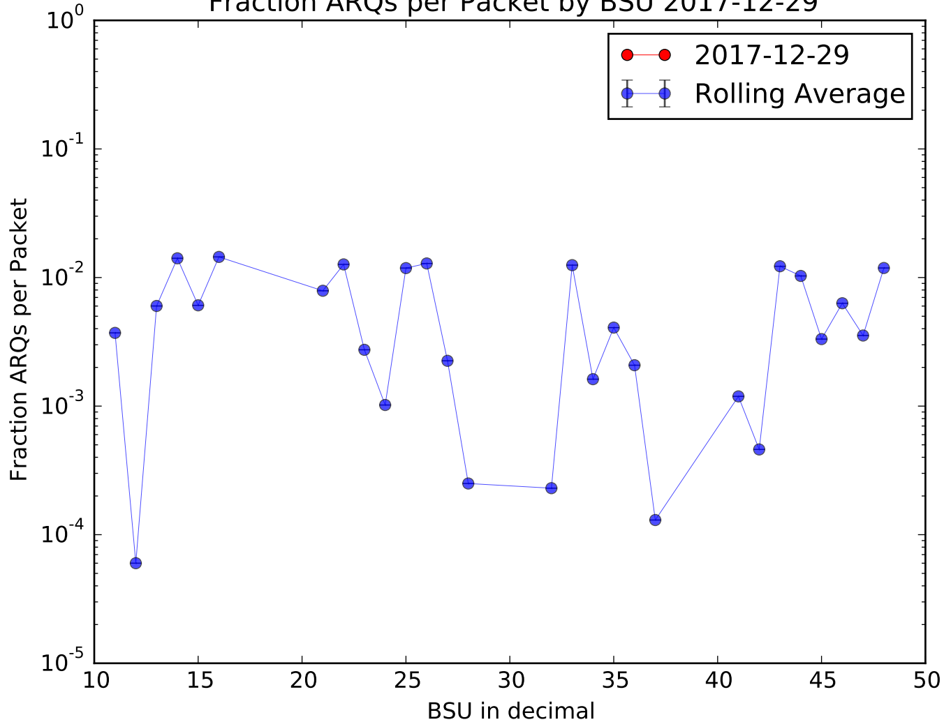
Fraction ARQs per Packet by BSU 2017-12-29
