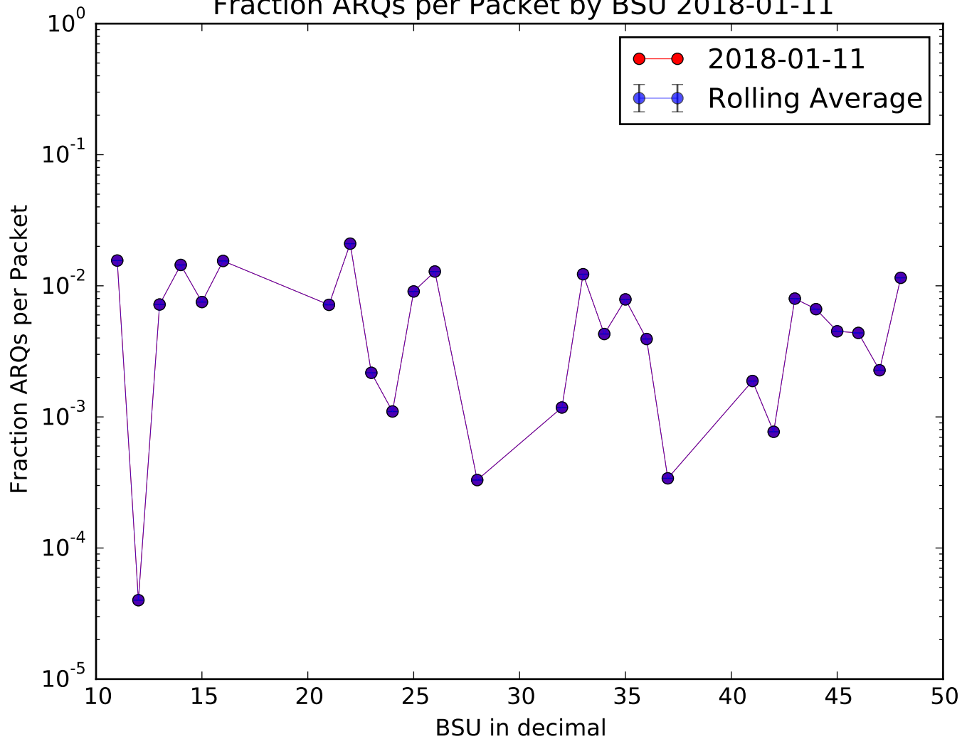
Fraction ARQs per Packet by BSU 2018-01-11
