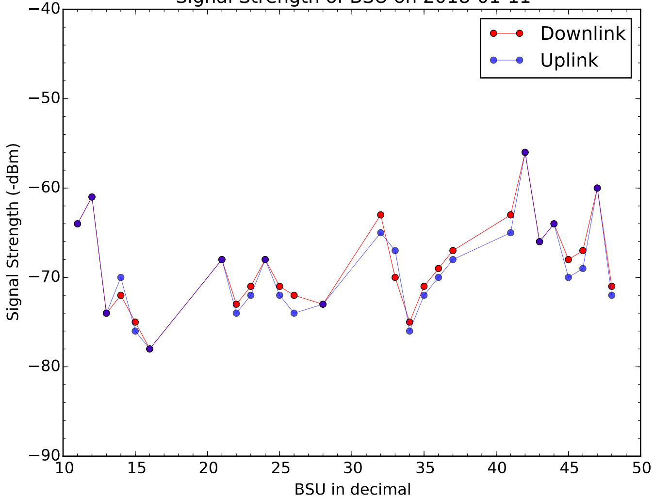
Signal Strength of BSU on 2018-01-11
