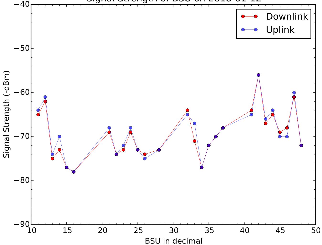
Signal Strength of BSU on 2018-01-12
