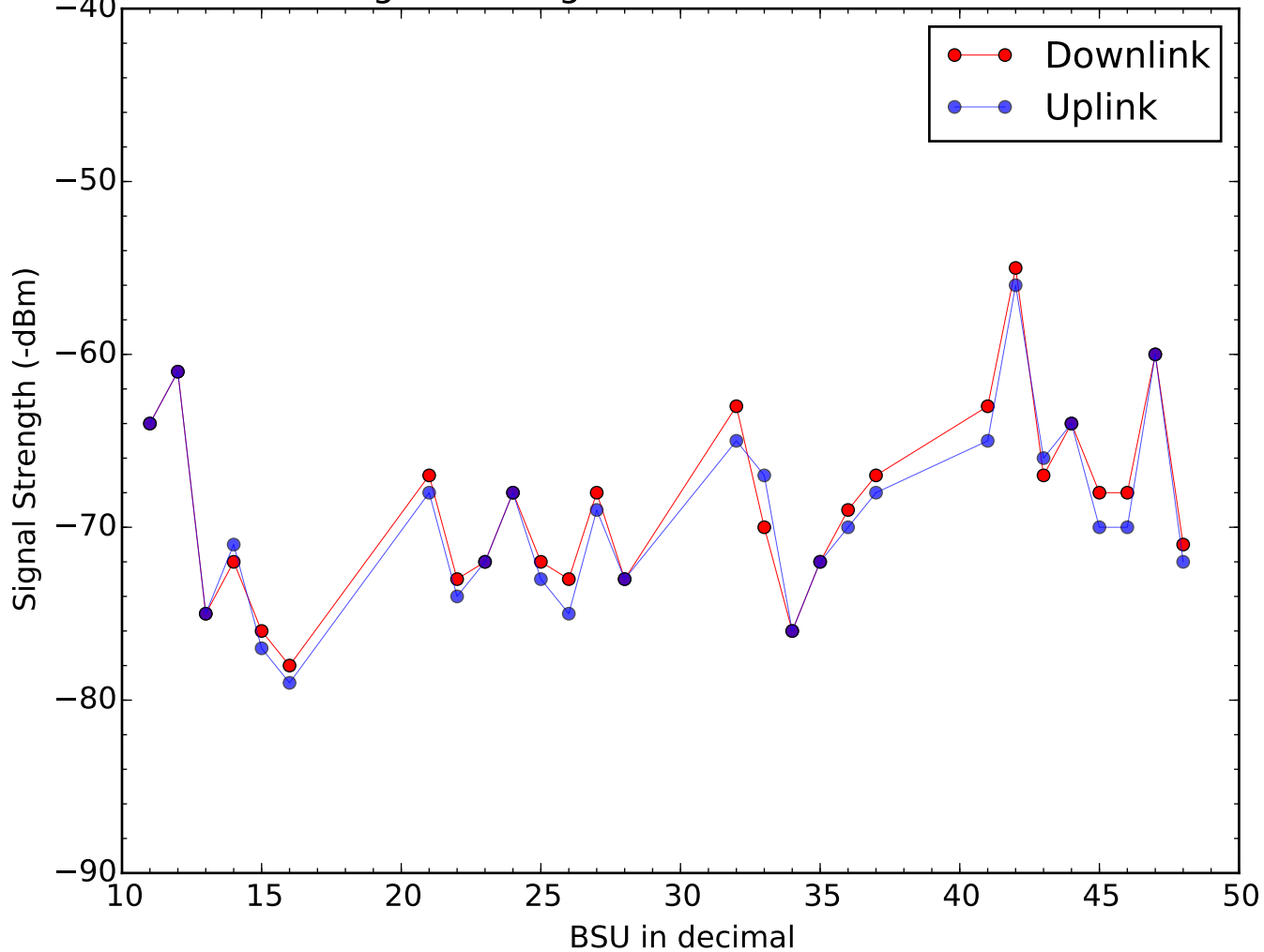
Signal Strength of BSU on 2018-01-16
