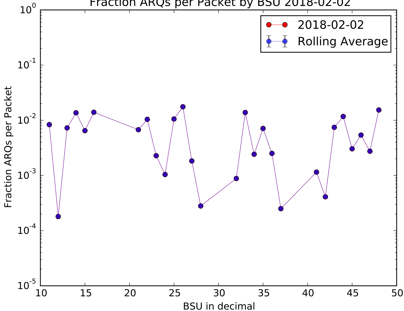
Fraction ARQs per Packet by BSU 2018-02-02
