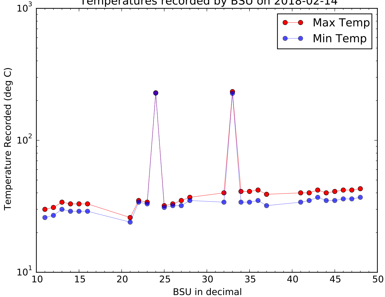
Temperatures recorded by BSU on 2018-02-14
