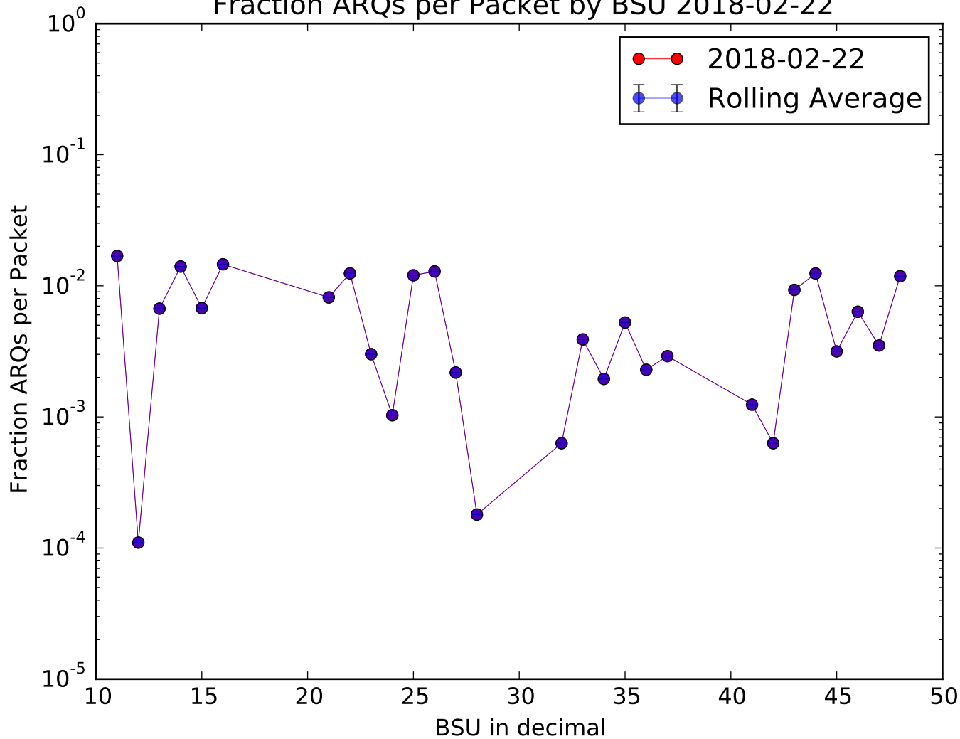
Fraction ARQs per Packet by BSU 2018-02-22
