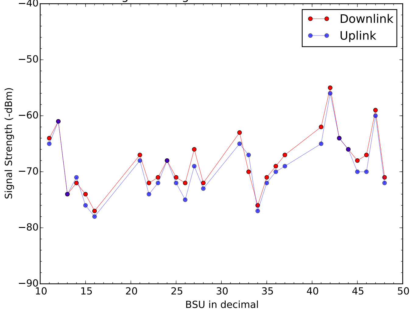
Signal Strength of BSU on 2018-02-24
