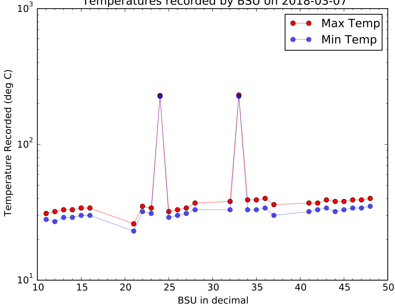
Temperatures recorded by BSU on 2018-03-07
