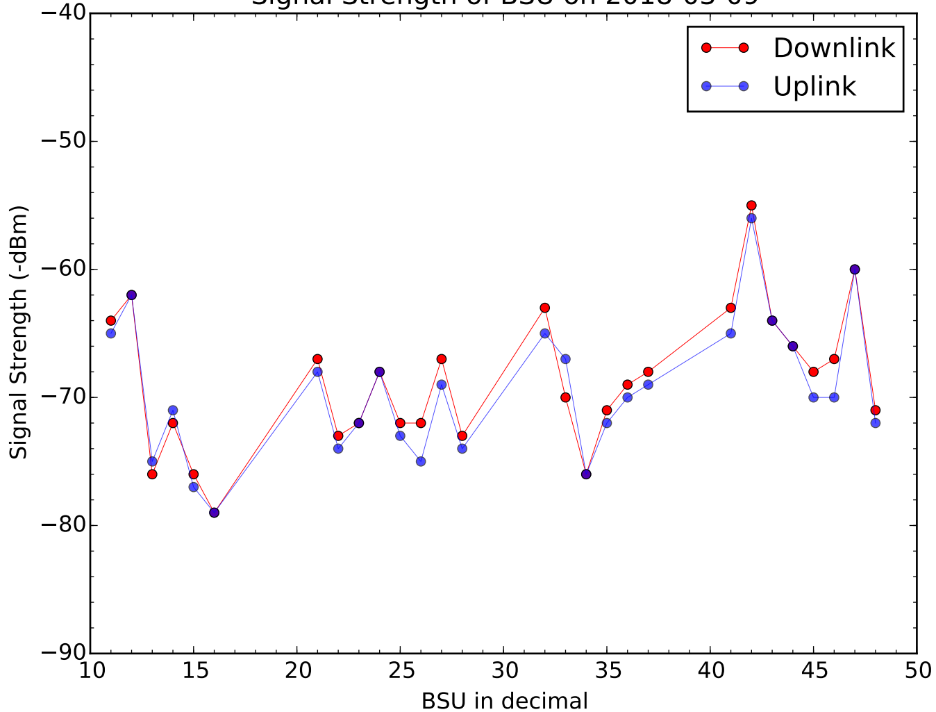
Signal Strength of BSU on 2018-03-09
