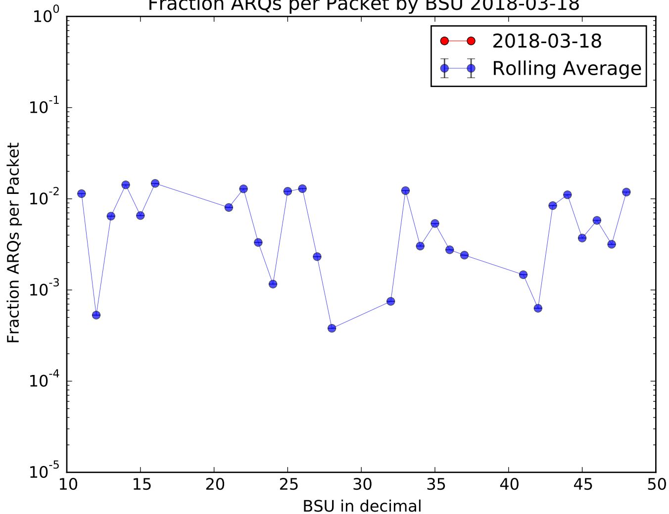
Fraction ARQs per Packet by BSU 2018-03-18
